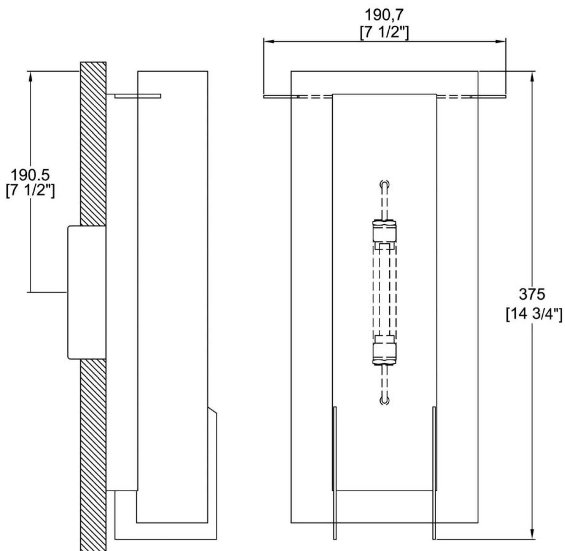
SIDE VIEW
